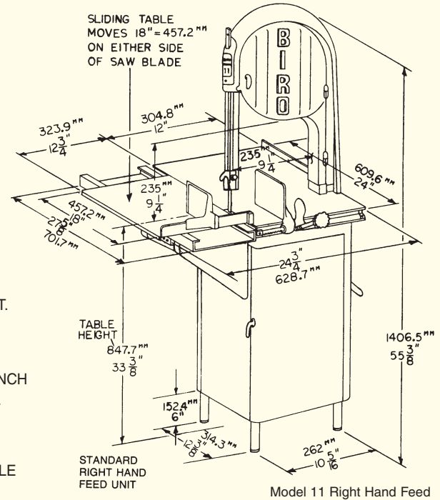
Model 11 Right Hand Feed
