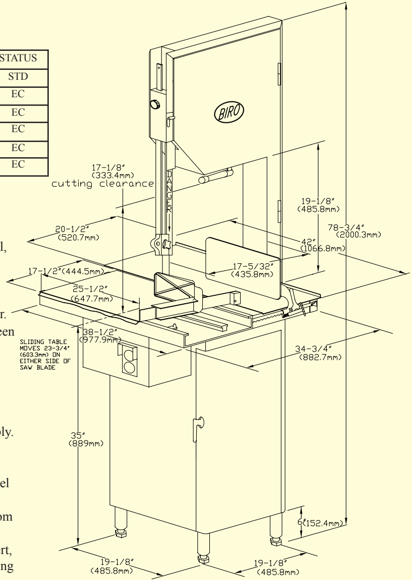
MODEL 44SSFH CONFIGURATION 142" (3606.8 mm) SAW BLADE
